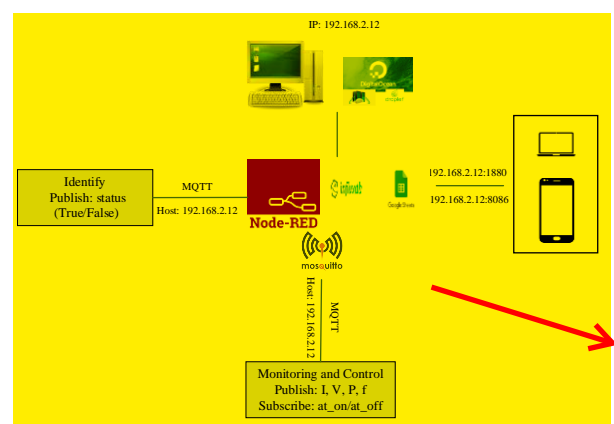
Figure 10. Diagram of data transmission and reception in the system.
