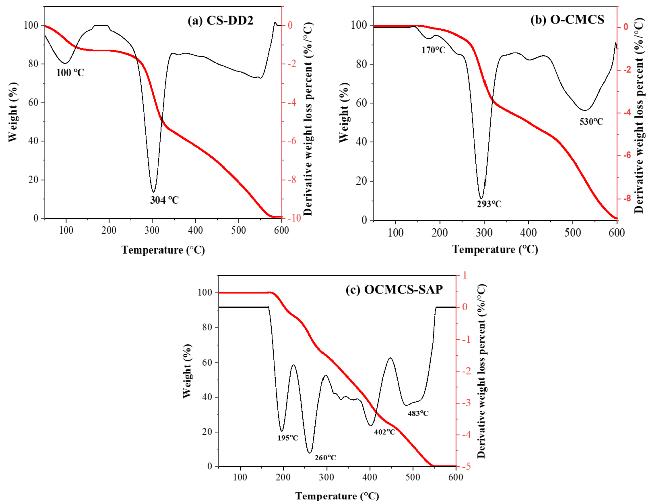
Figure 14. TGA results of CS-DD2, O-CMCS, and OCMCS-SAP
